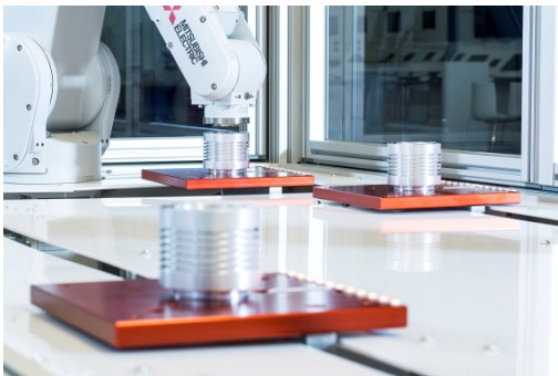
Picture 2: The Smart Carriage also supports the ability to switch between parallel tracks on production lines allowing multiple operations on different products.
